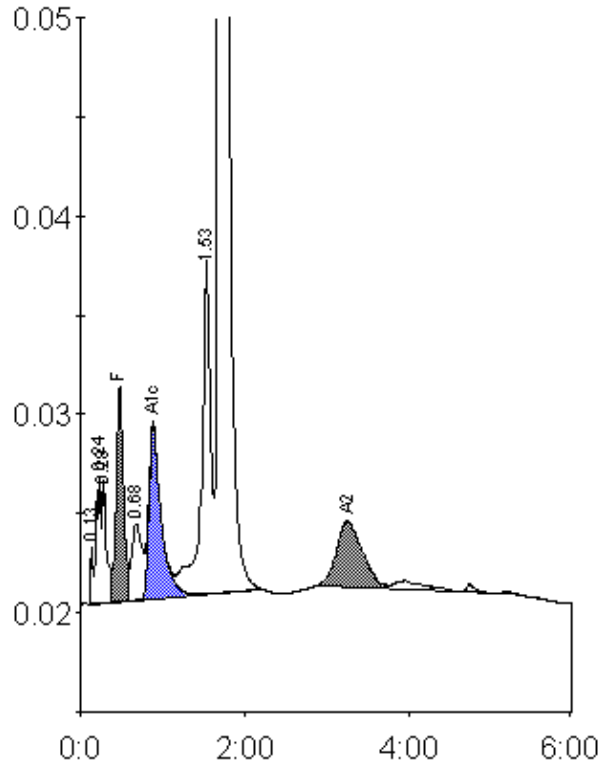
Peak table - ID: 10532864
